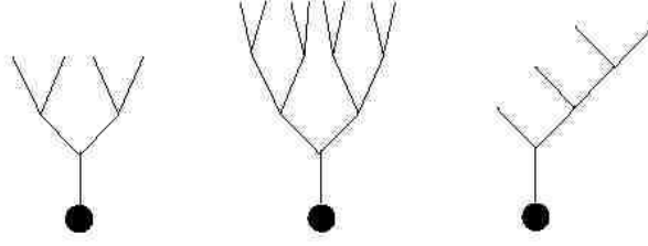
FIGURE 4. The symmetric trees of height 2 and 3, and a non-symmetric tree of class 4
